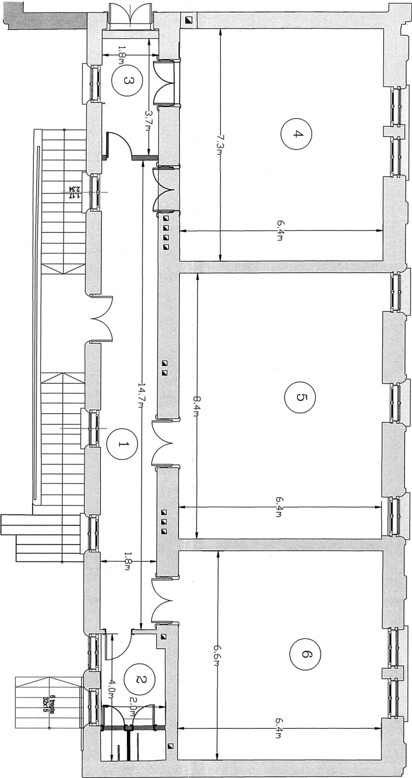
C5 - Plan Parter
