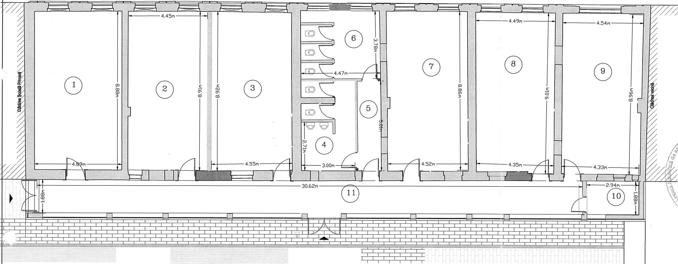
C3 - Plan parter
