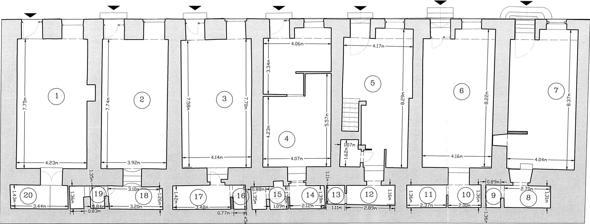
C3 - Plan Demisol
