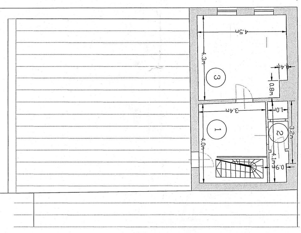
C8 - Plan mansardă
